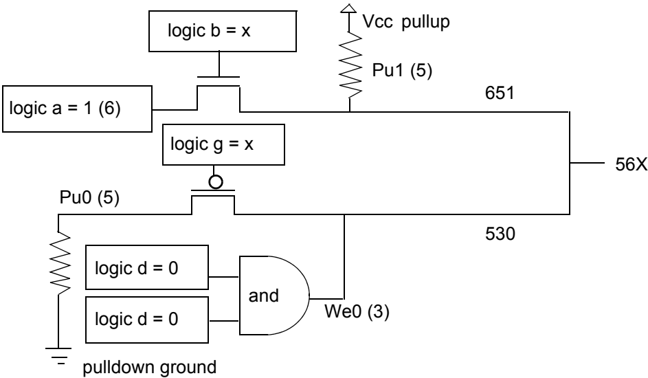
Figure 28-11—Ambiguous strengths from switch networks
